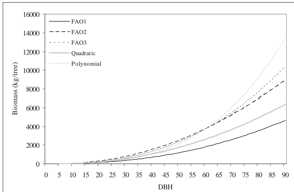
Figure 4 Allometric equations for estimating biomass of tropical trees. FAO1, FAO2 and FAO3 were developed by Brown (Brown, 1997), whilst Quadratic and Polynomial were developed by Mbow (Mbow, 2009).
